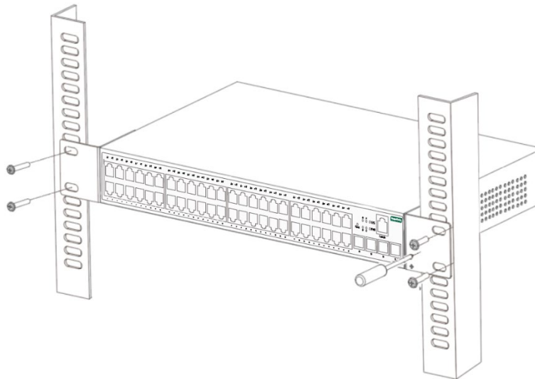
Figure 3-3 Diagram 2 of rack installation
