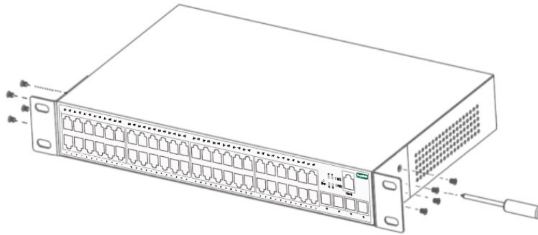
Figure 3-2 Diagram 1 of rack installation
